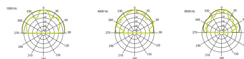
HORIZONTAL / VERTICAL POLAR DIAGRAMS
