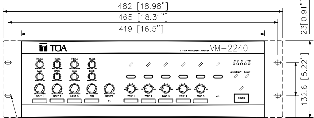
Front View
