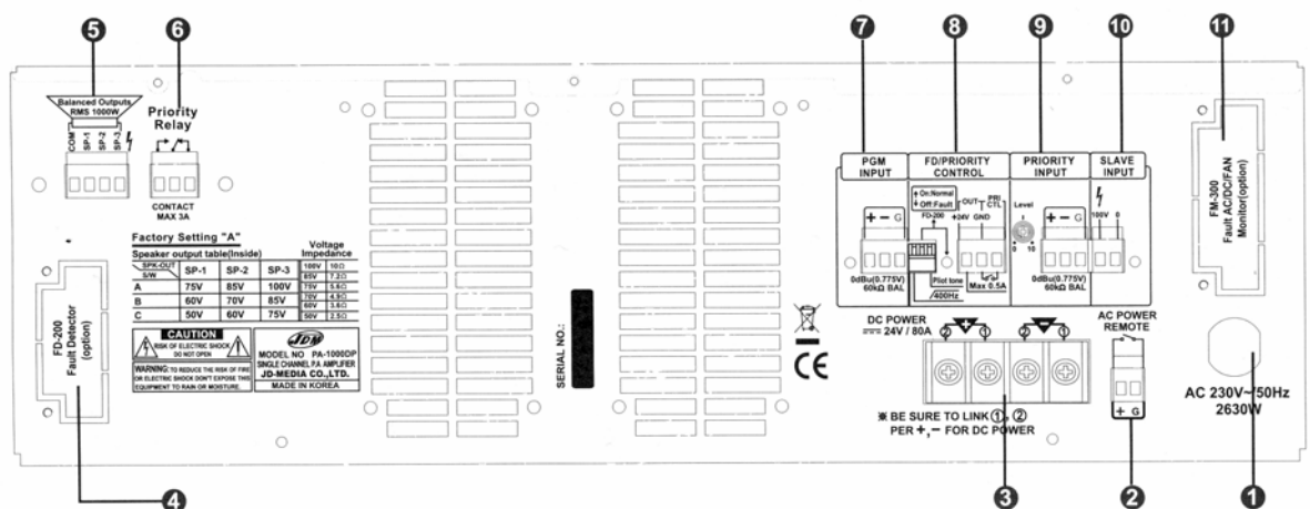
PA-1000DP
