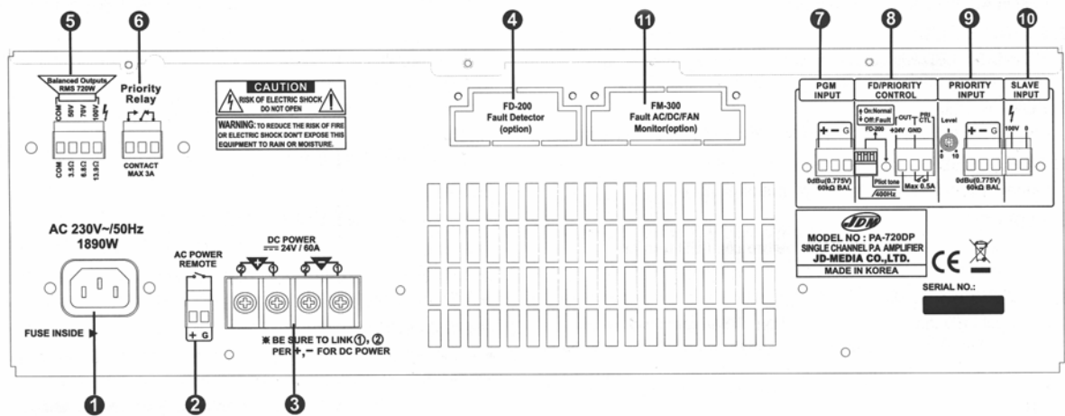
PA-600/720DP
